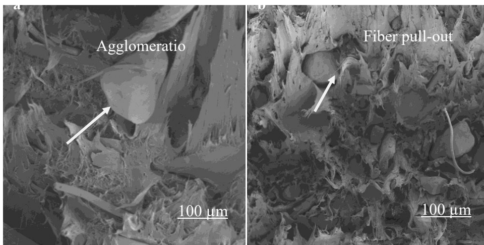
Plate 3a: SEM micrographs 150 μm of GHP-PLA composites
