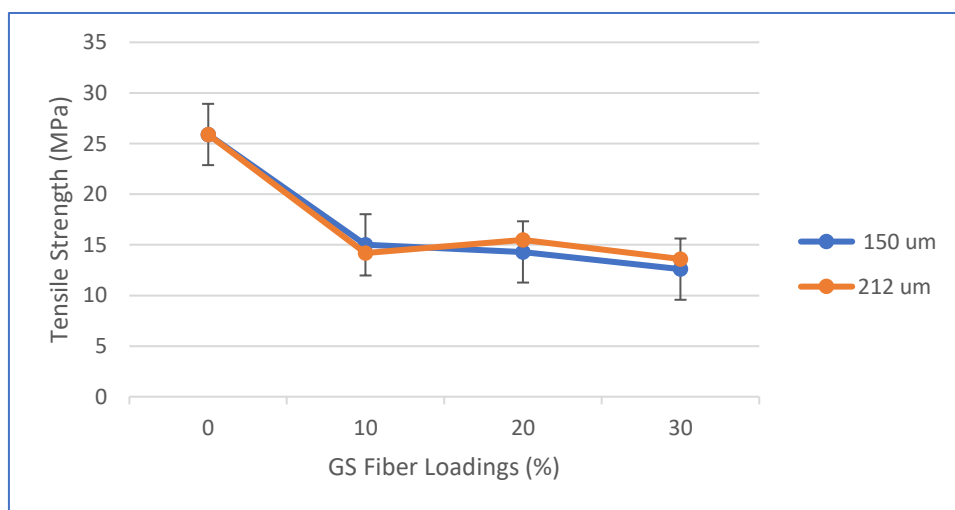
Figure 3: Effect of fiber loading on the tensile strength of GSP-PLA Composite
