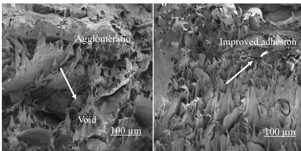
Plate 3b: SEM micrographs 212 μm of GHP-PLA composites
