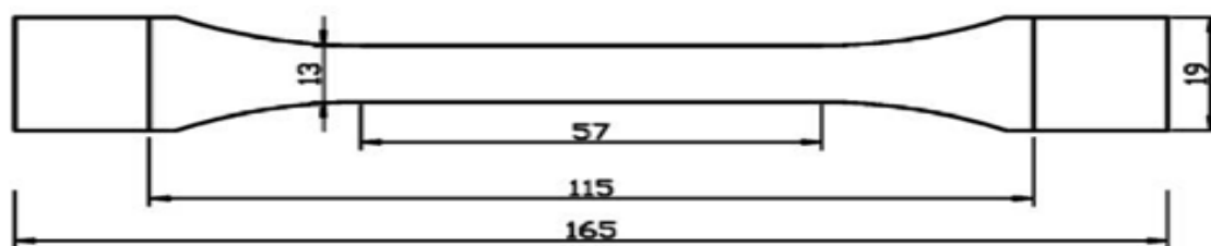
Figure 2: Tensile test specimen as per ASTM D638
