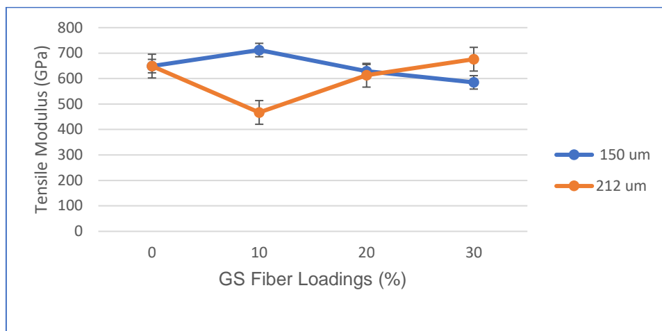
Figure 4: Effect of fiber loading on the tensile modulus of GSP-PLA Composite
